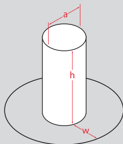
Pipe Boot
